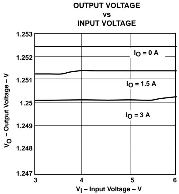
Figure 2–5. Line Regulation
